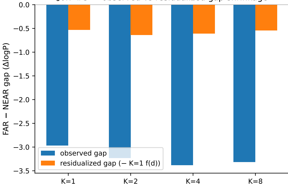
§6.7 #3 — observed vs residualized gap-shrinkage
