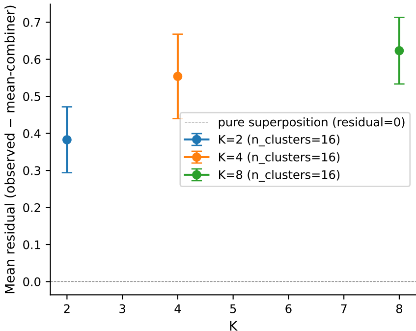
Level-1 superposition residual per K (cluster-robust 95% CI)
