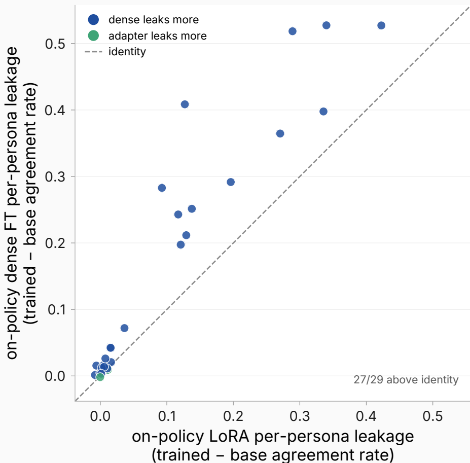
villain round 4: dense vs adapter per-persona leakage ( \rho=0.93 , n=29 )
