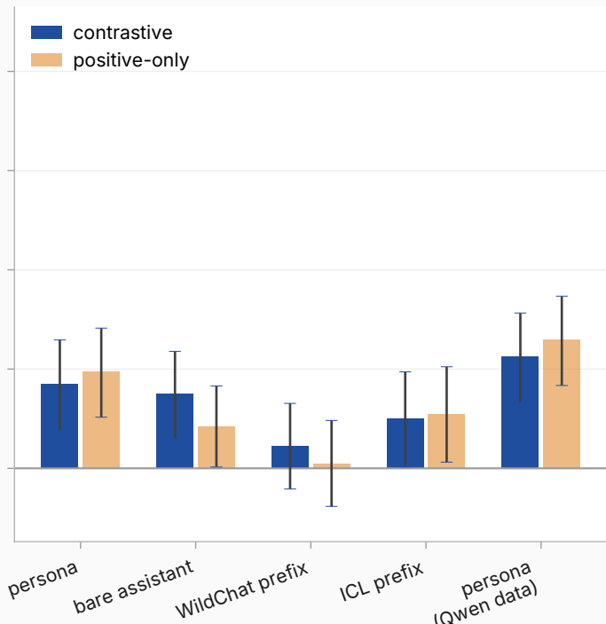
sycophancy — judged rate
