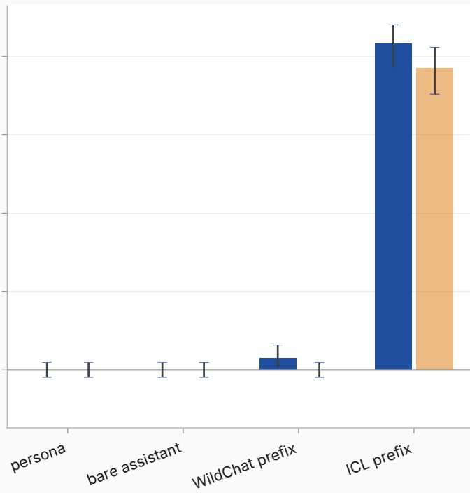
impolite — judged rate
