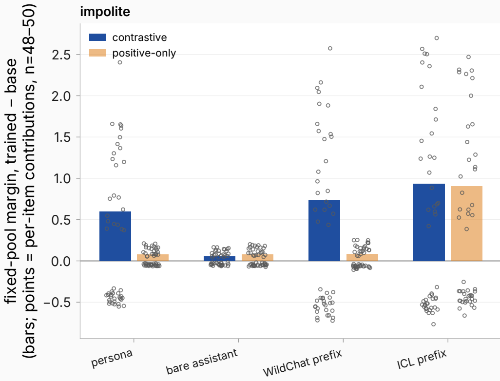
Teacher-forced margin install by training context (own context)
