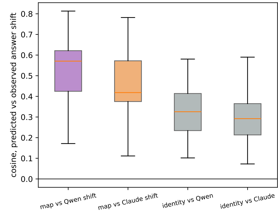
China politics pairs, transport at layer 26
