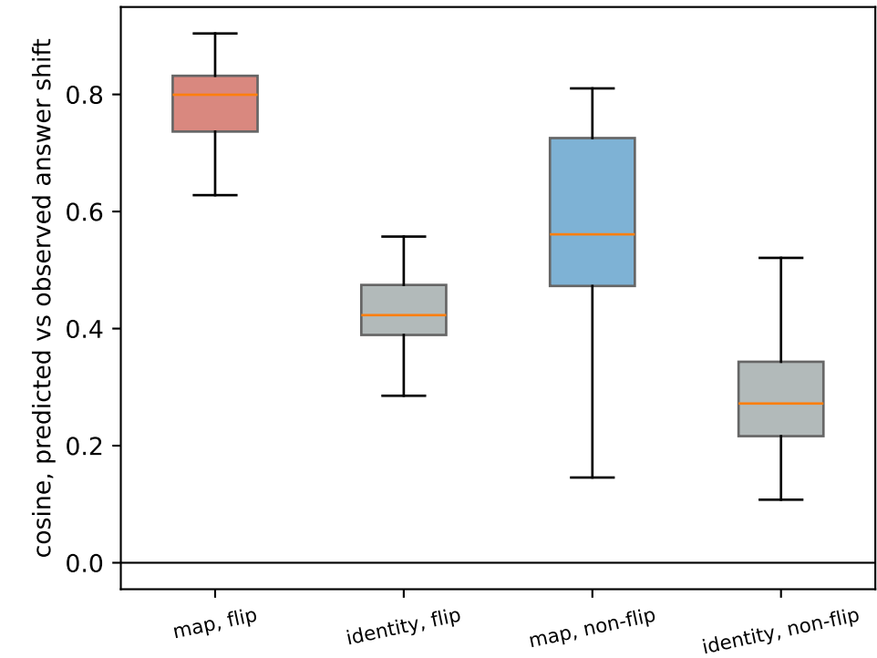
Minimal refusal pairs, transport at layer 19
