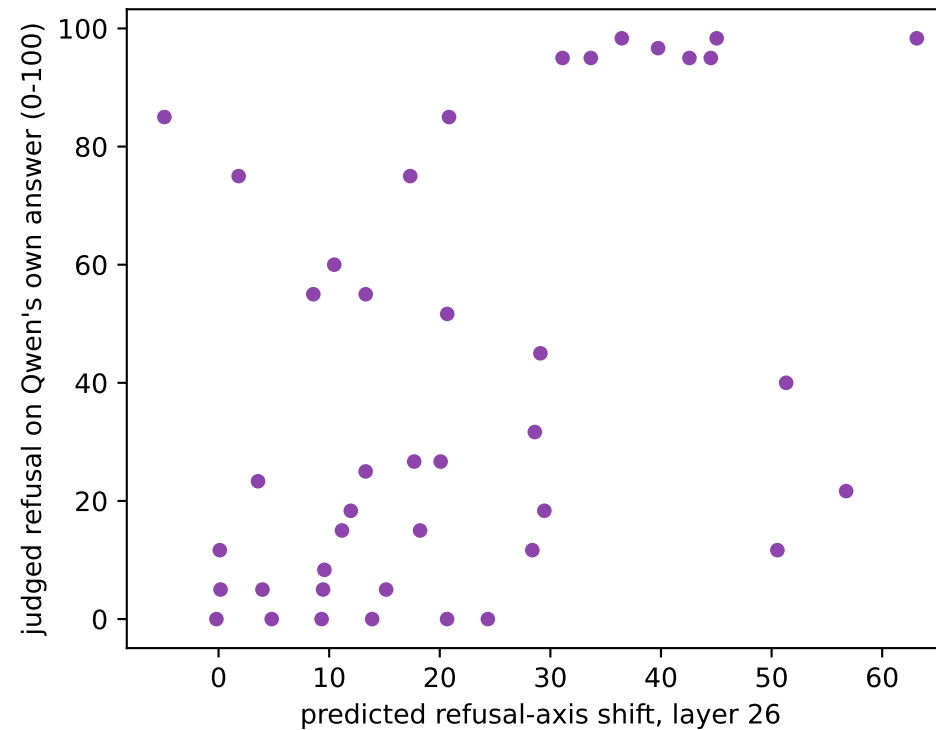
China politics pairs
