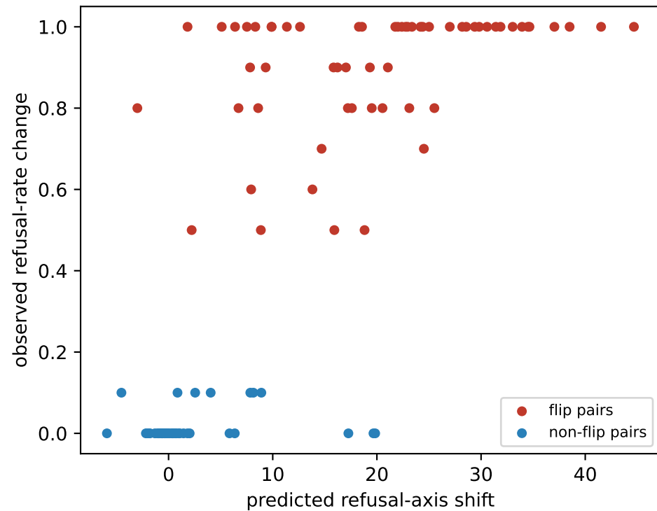
Minimal refusal pairs, layer 19
