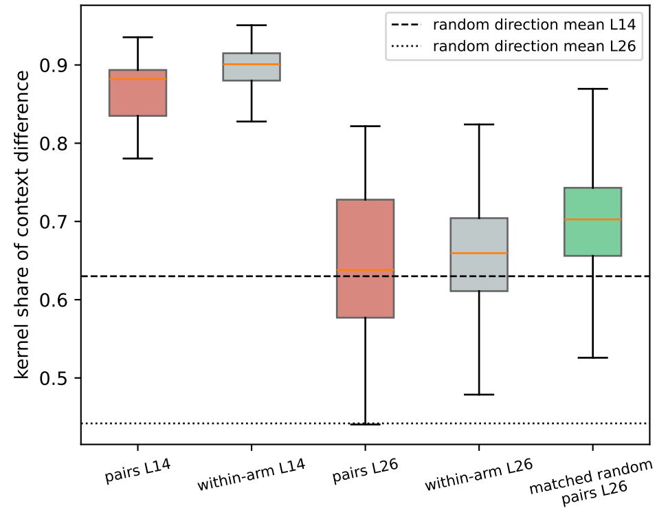
China politics pairs, layers 14 and 26
