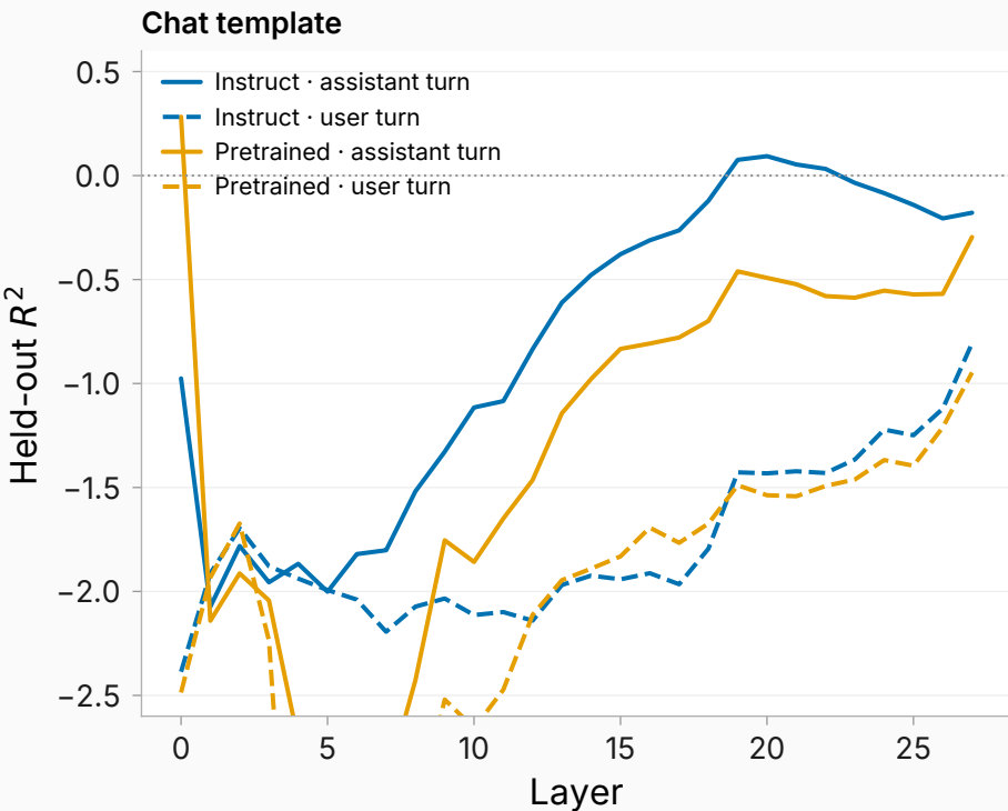
Two-turn track: held-out R^2 by layer, assistant vs user turn
