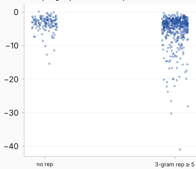
instruct: per-group rotated R^2 vs repetition
