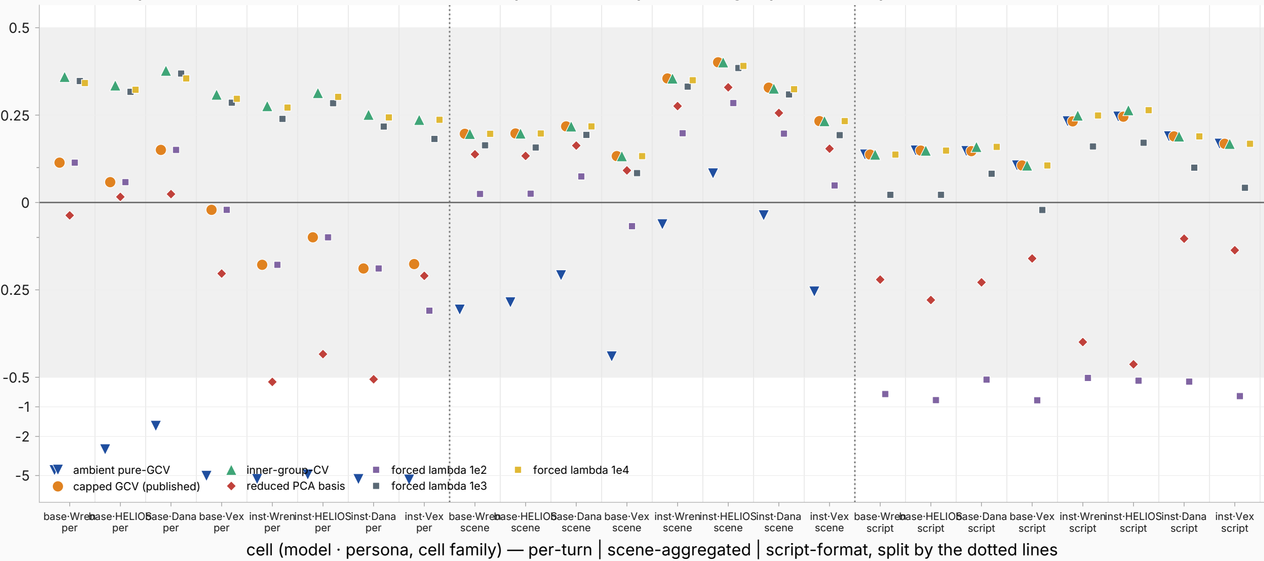
Held-out R^2 per cell under each lambda selector — ambient pure-GCV collapses, inner-group-CV lifts the per-turn cells
