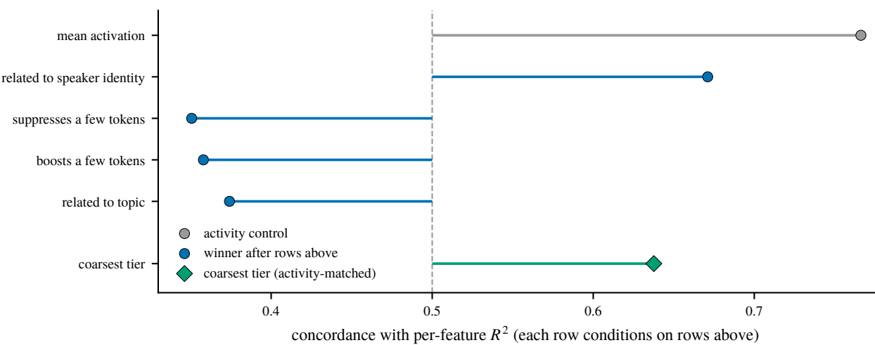
Figure 5. Forward-stepwise partialling: each row conditions on all rows above. c = concordance (AUROC scale), 0.5 = chance. Gray: activity control. Diamond: matryoshka coarsest tier different dictionary, direction only. No CIs; later rounds omitted.
