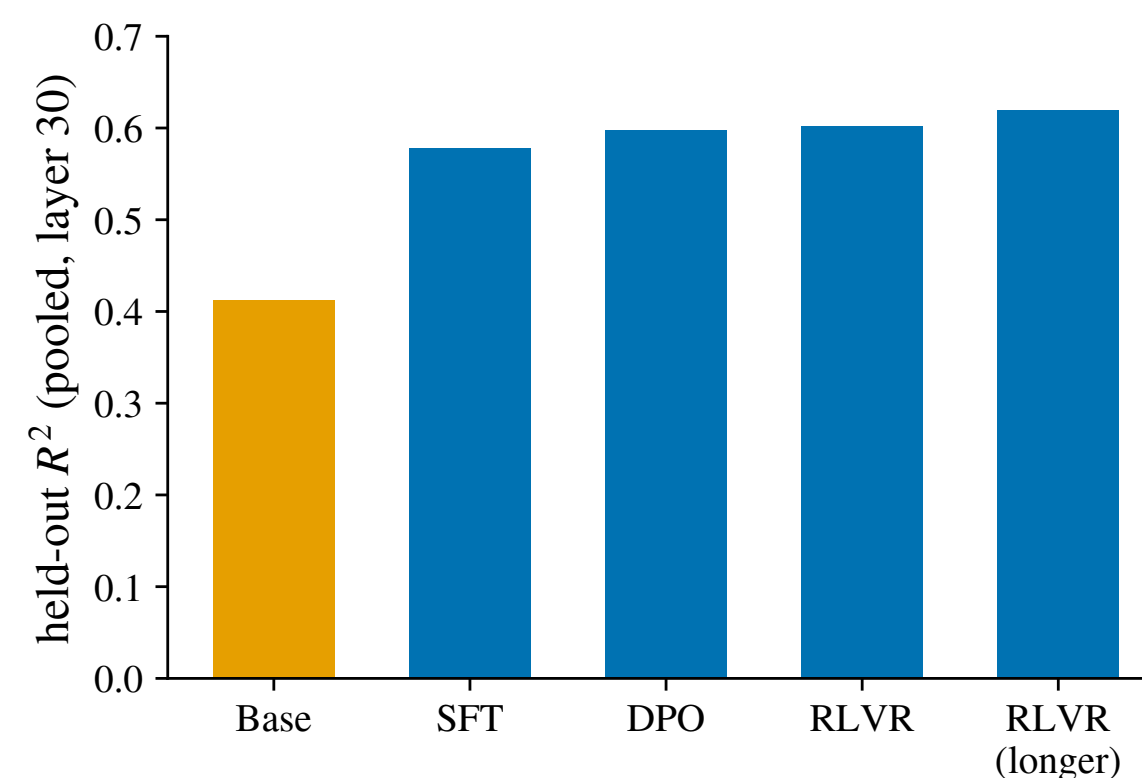
Figure 7. Pooled held-out R^2 at each stage of the Llama/Tülu ladder (layer 30), each stage fit and evaluated on its own on-policy answers.
