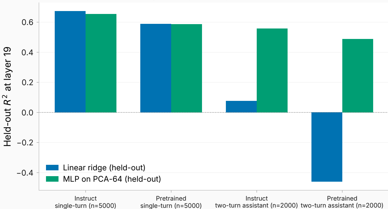
Linear ridge vs MLP map strength at layer 19
