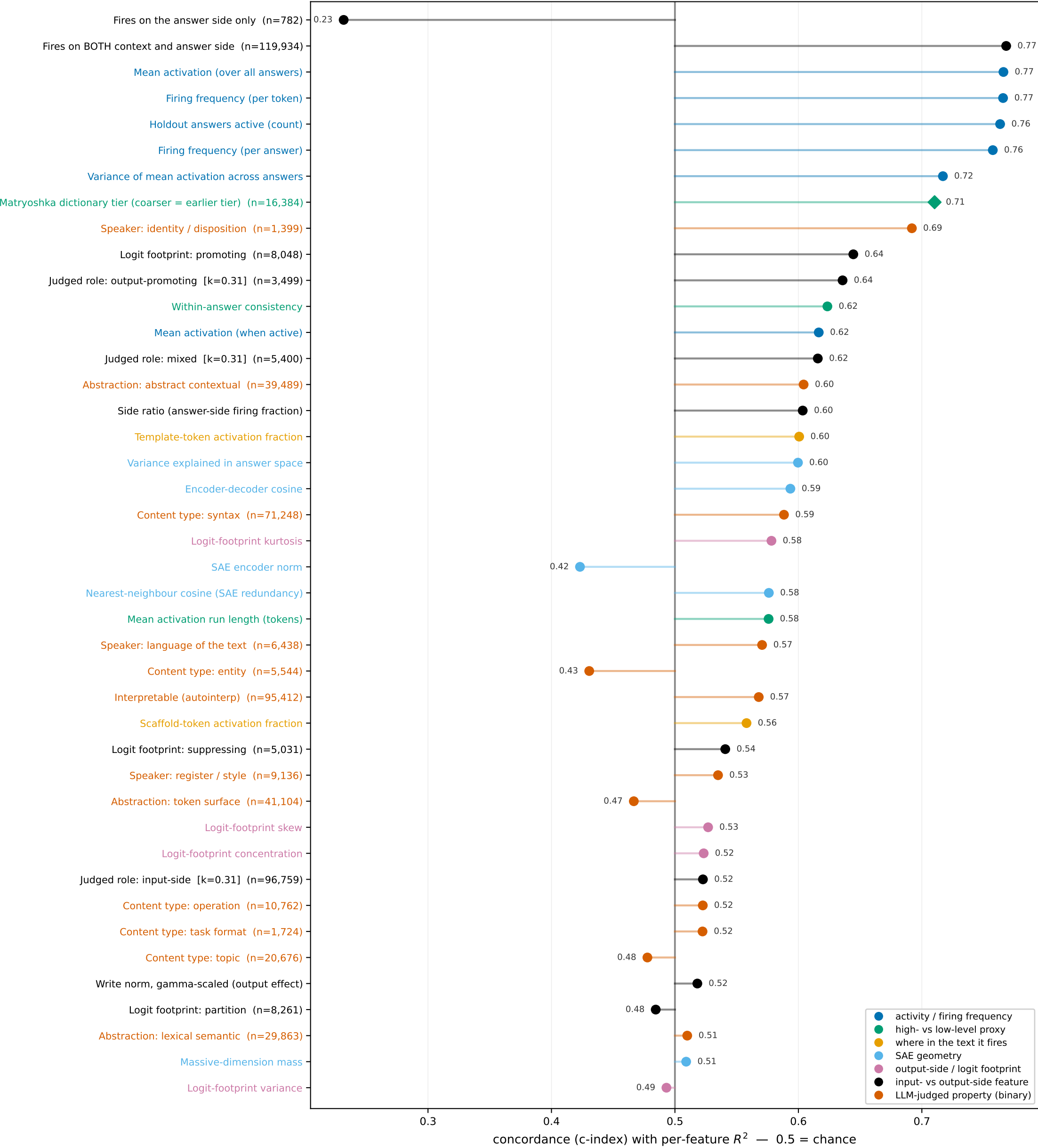
Which feature properties predict how well the context→answer map predicts a feature? concordance over all pairs · sorted by predictive power |c - 0.5| \cdot n = 120,716 features
