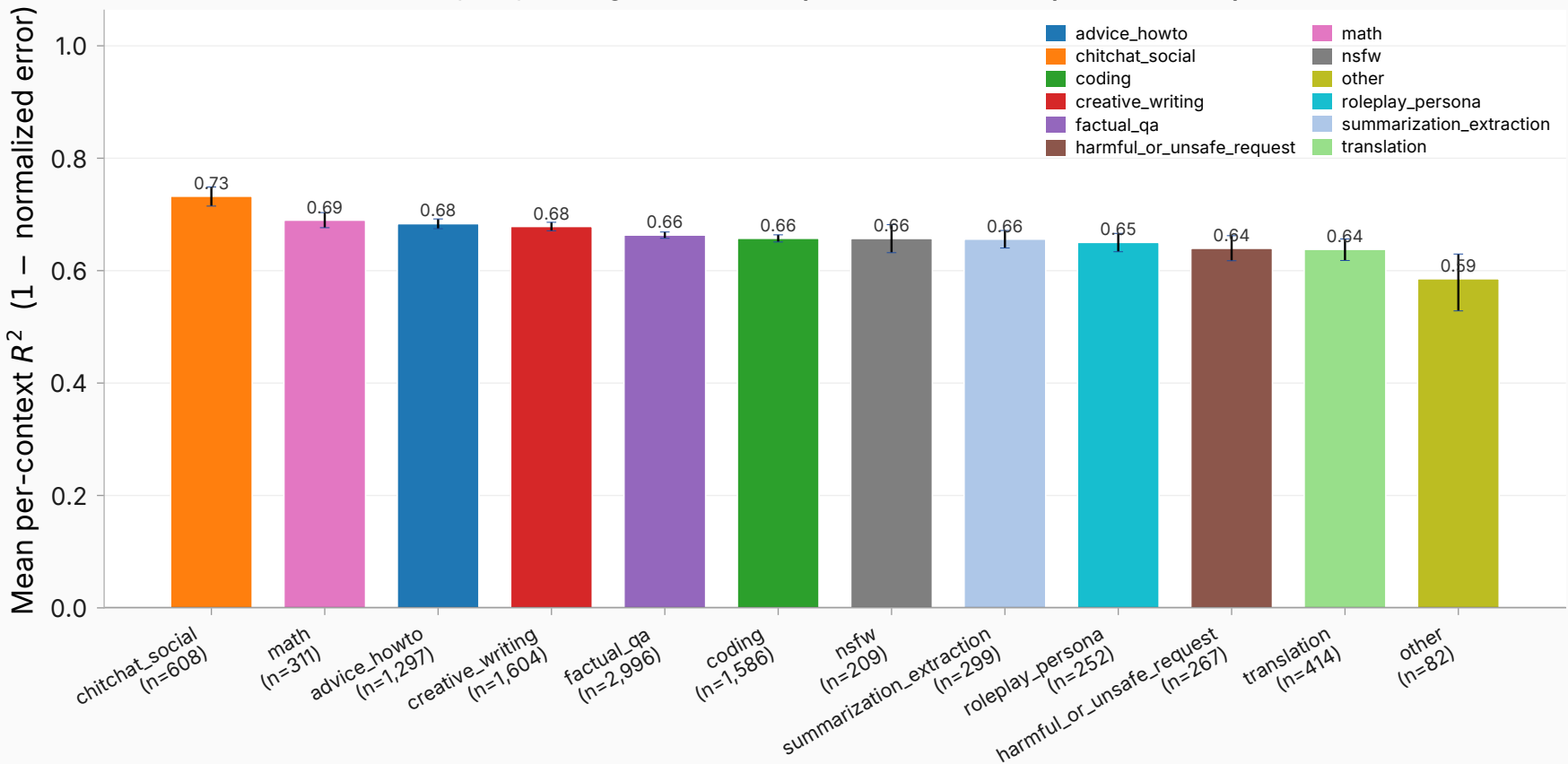
Context vector → answer: prediction quality by judged context category #1738 multi-turn holdout (n=9,941), L19 ridge · sorted best-predicted first · 95% paired bootstrap CI
