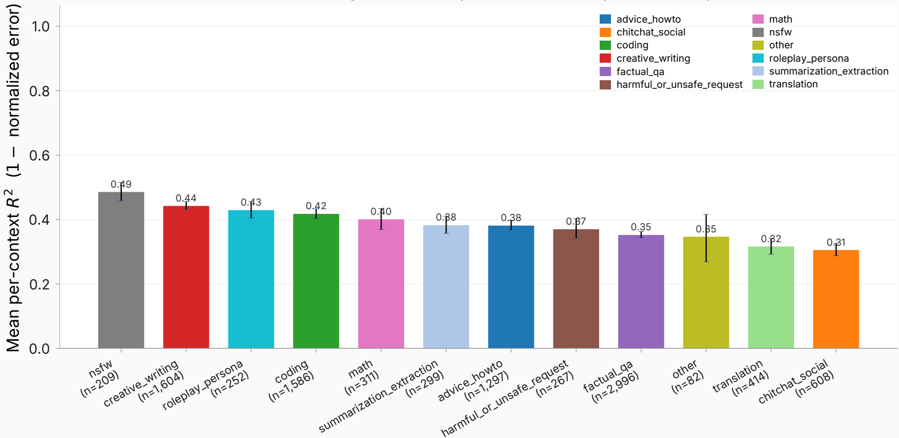
Prefix end state → answer: prediction quality by judged context category #1738 multi-turn holdout (n=9,941), L19 ridge · sorted best-predicted first · 95% paired bootstrap CI
