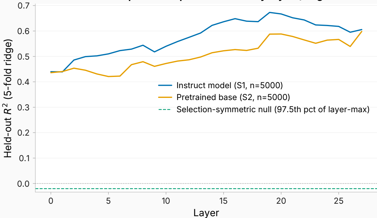
Context→answer-profile map: held-out R^2 by layer (single-turn track)
