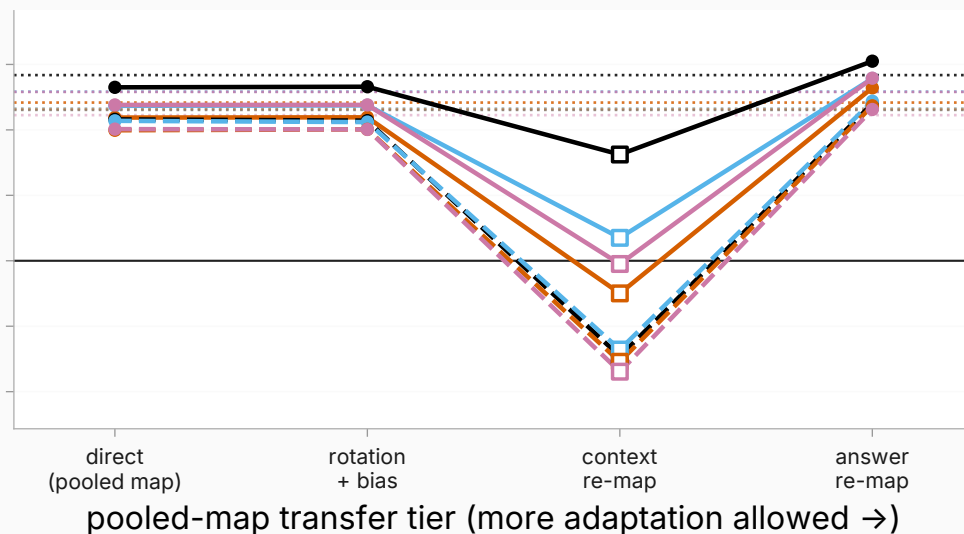
Qwen2.5-7B-Instruct
