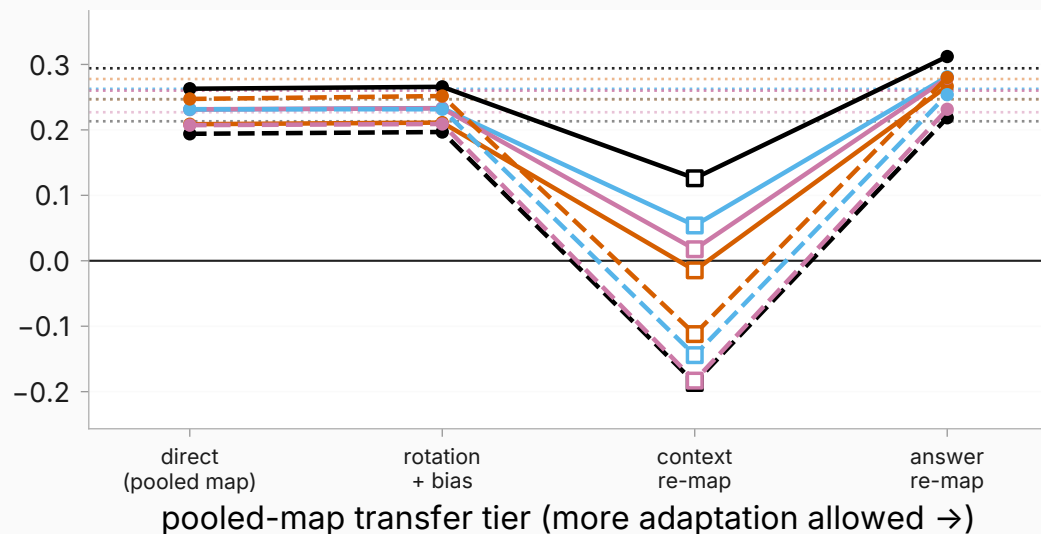
Qwen2.5-7B (base)
