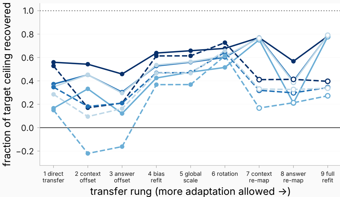
Qwen2.5-7B (base)
