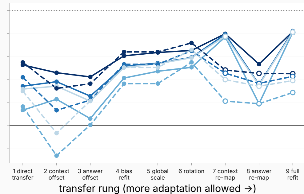
Qwen2.5-7B-Instruct
