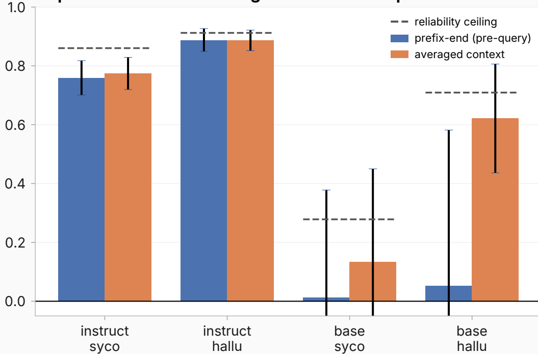
Supervised read of average behavioral disposition vs its reliability ceiling
