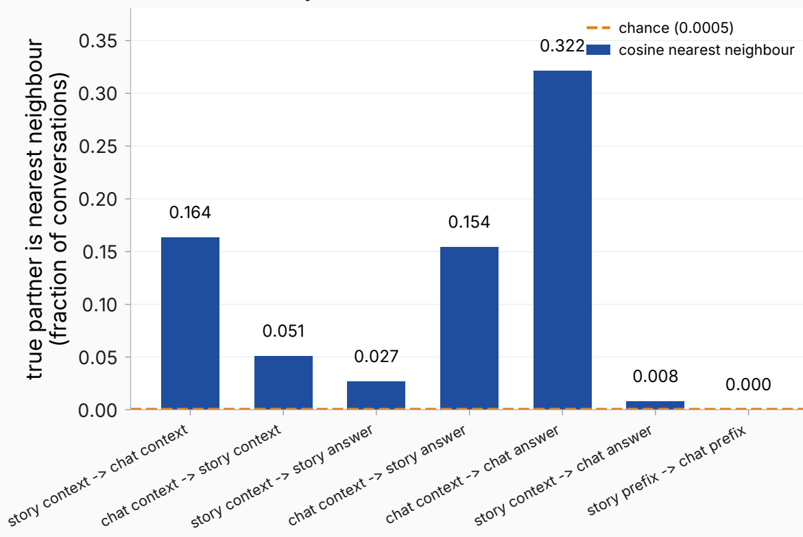
Raw retrieval, no fitted map, layer 19 teacher-forced story (n=2163)
