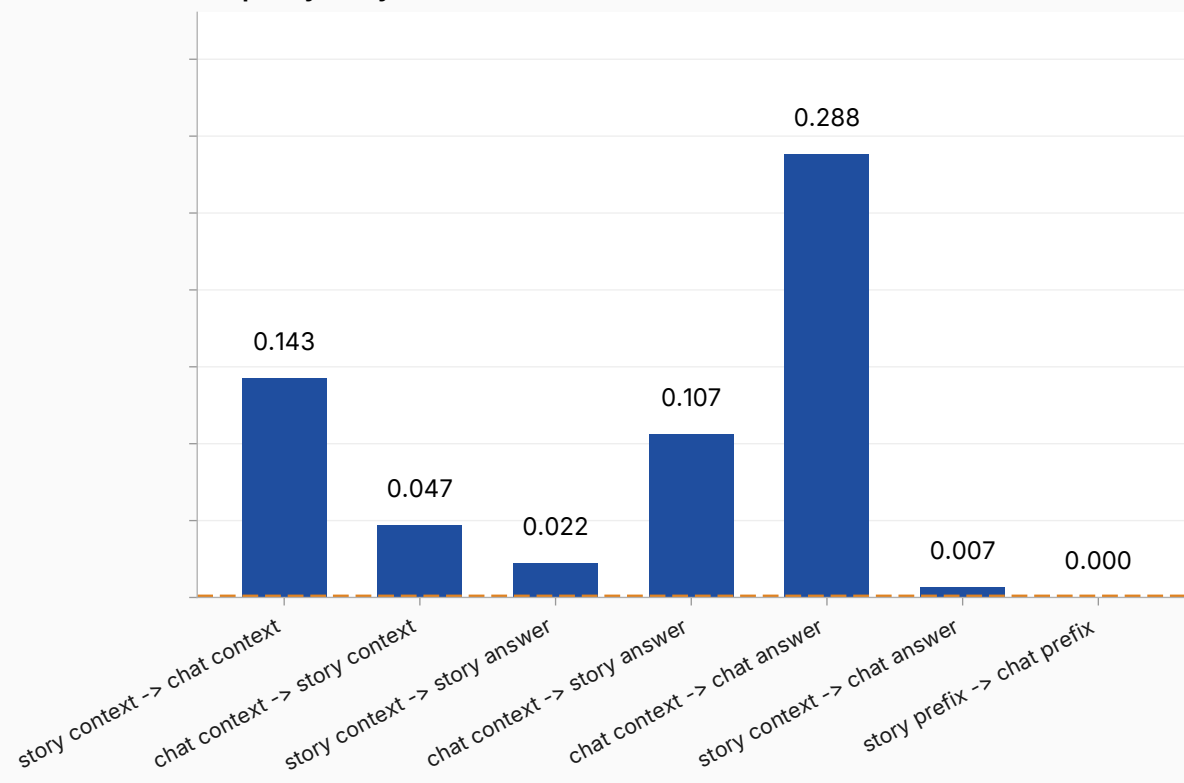
Raw retrieval, no fitted map, layer 19 on-policy story (n=2018)
