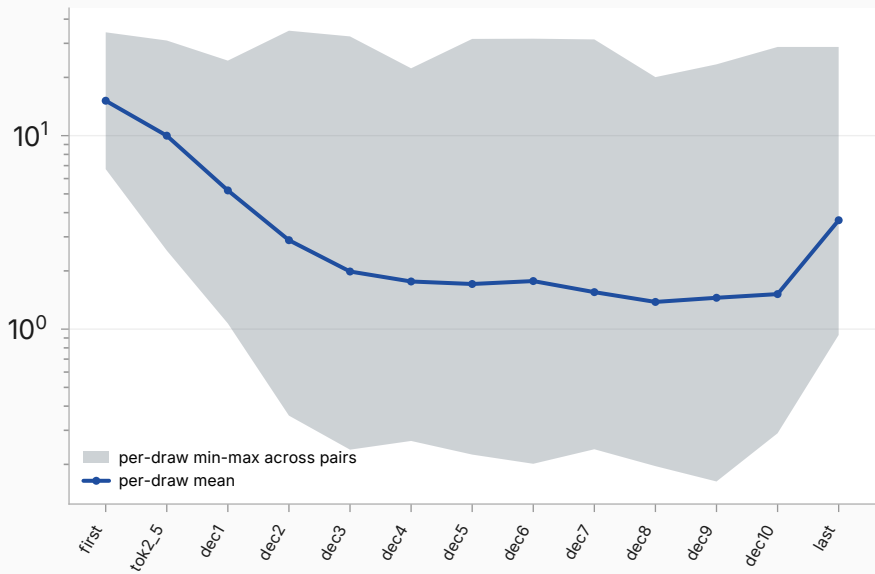
per-draw dispersion — steered/context/L14 (read L17)
