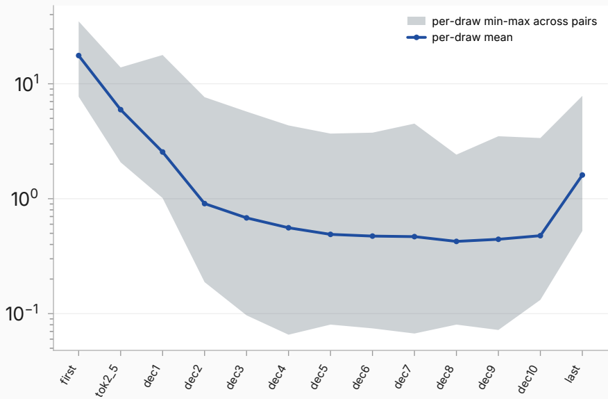
per-draw dispersion — steered/context/L20 (read L21)
