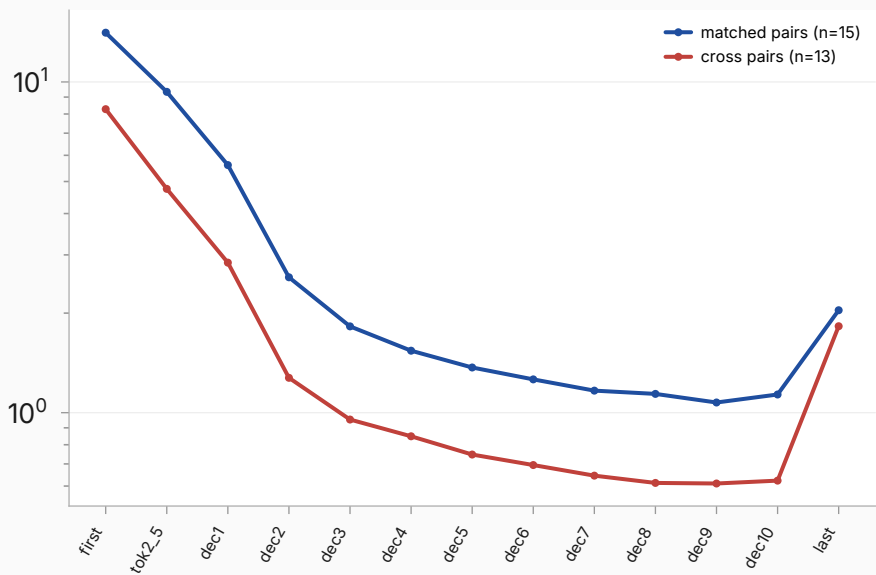
matched vs cross — steered/prefix/L14 (read L17)
