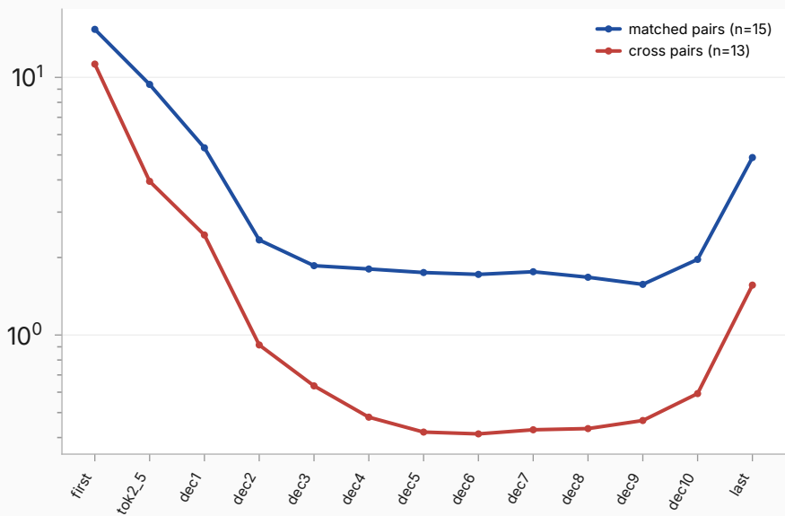
matched vs cross — steered/prefix/L20 (read L21)
