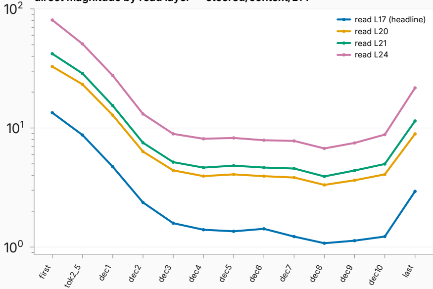
direct magnitude by read layer — steered/context/L14
