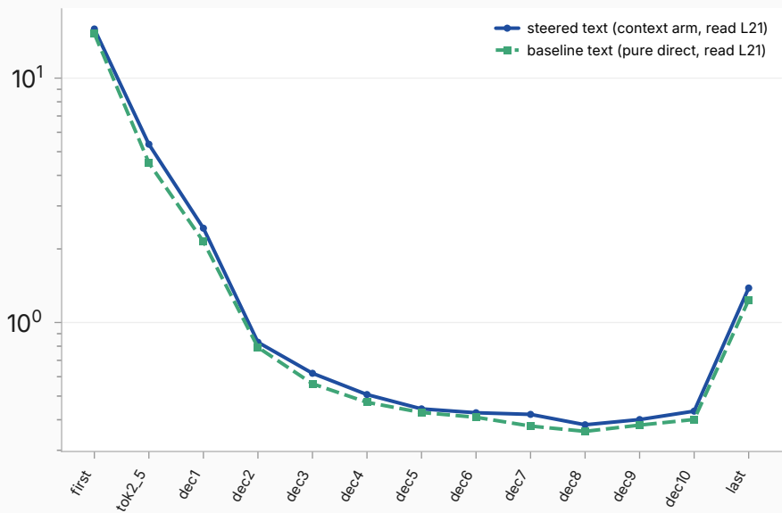
steered vs baseline text direct component — steer L20
