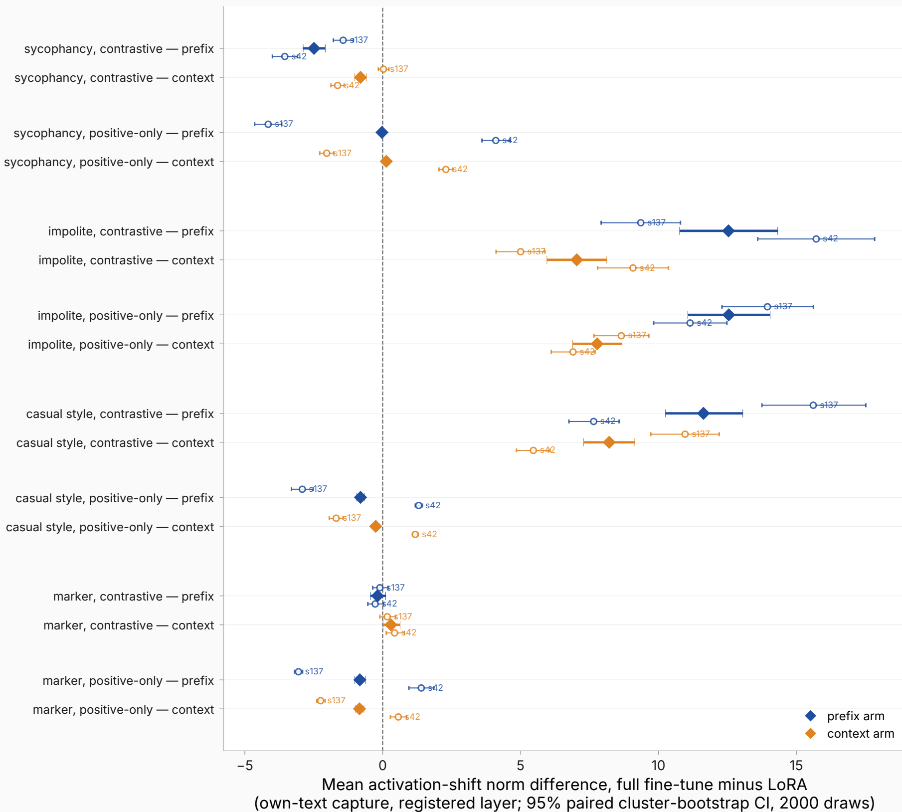
Prefix-arm vs context-arm method contrast (full fine-tune minus LoRA) (diamond = seed-pooled; labeled open circles = per-seed cells)
