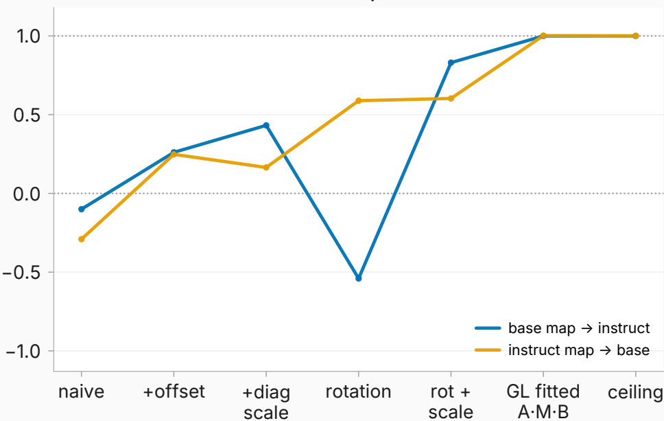
C — character 4×4, instruct (#1310/#1639)
