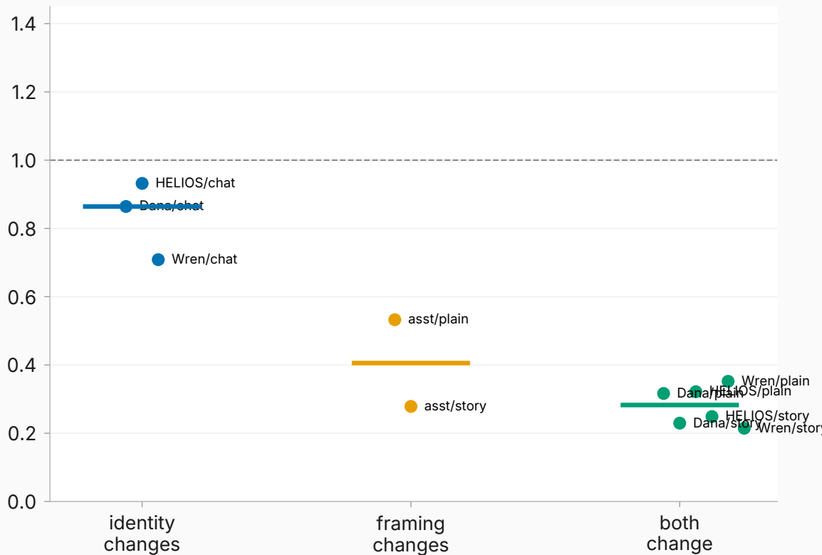
context arm
