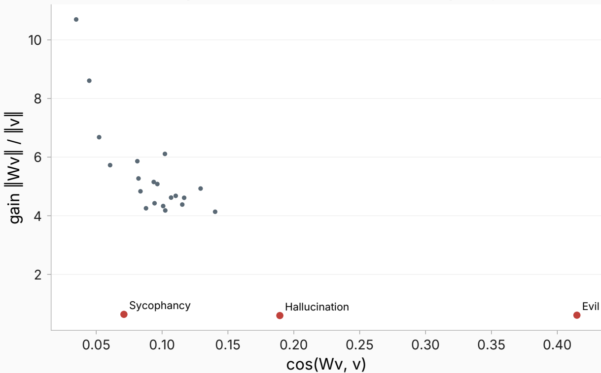
Preservation map: trait directions (labeled) vs top singular directions
