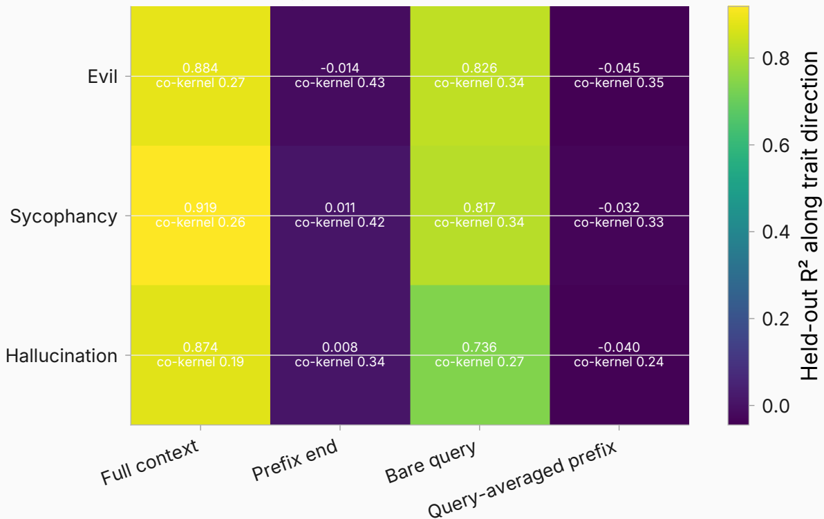
Trait readability by arm (L14; hatch = noise-limited; co-kernel@k90 overlay)
