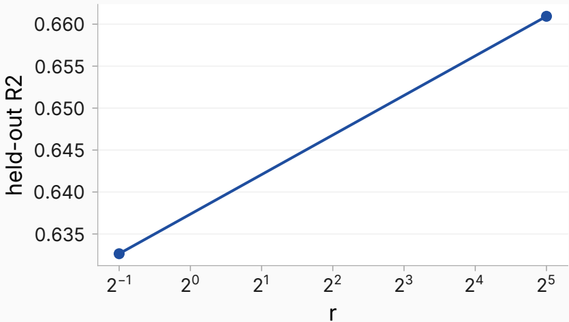
bilinear r-curve (doubly; exploratory)
