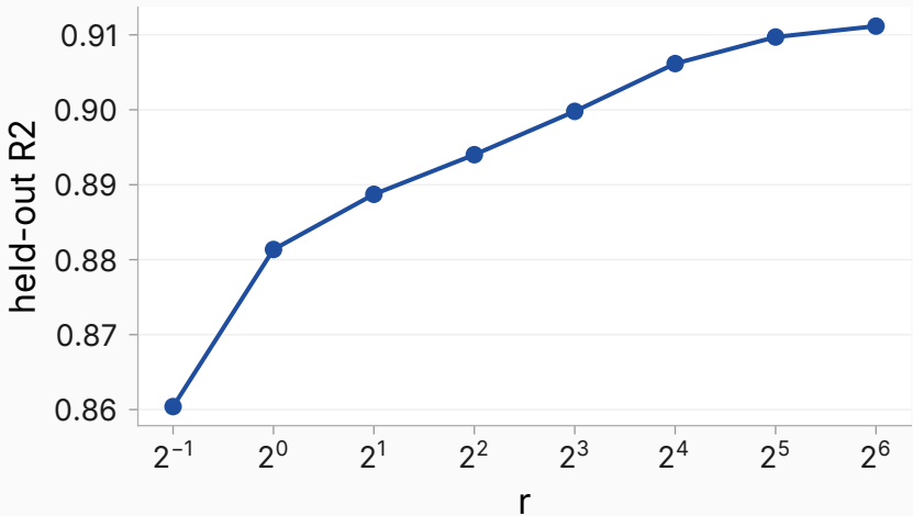
bilinear r-curve (prefix; exploratory)
