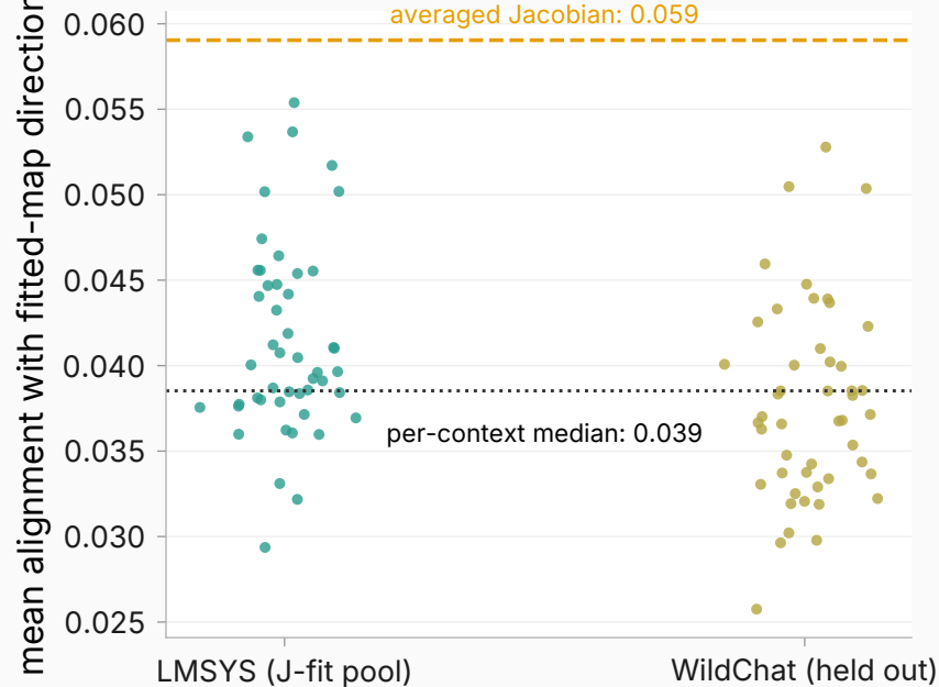
Alignment with the fitted map: no better per context
