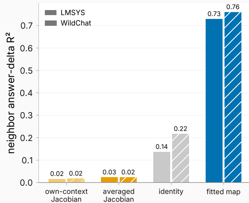
Even a context's own Jacobian predicts ~nothing
