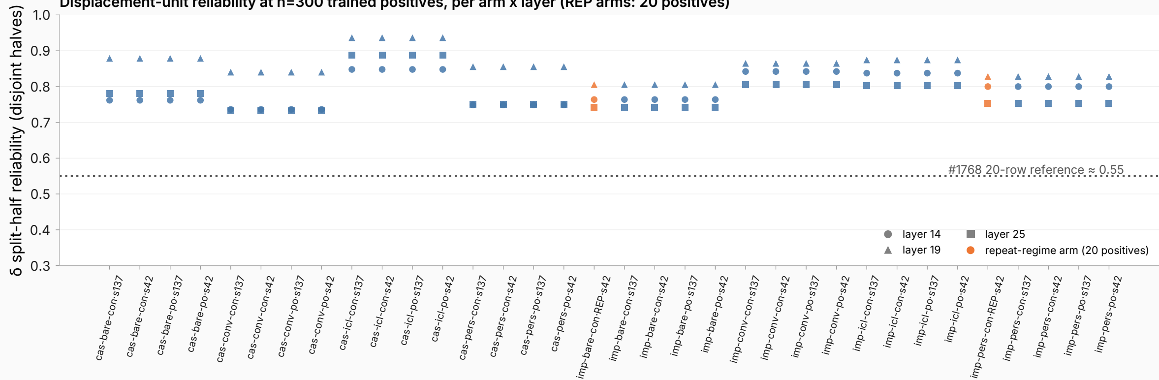
Displacement-unit reliability at n=300 trained positives, per arm x layer (REP arms: 20 positives)
