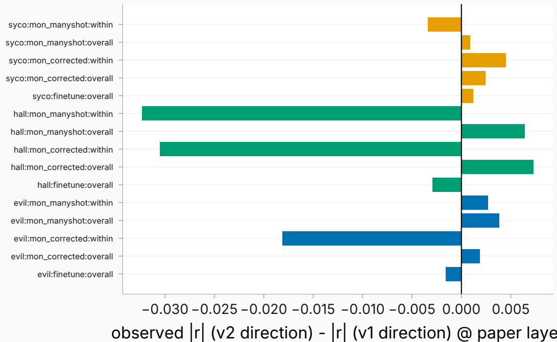
Extraction-fidelity impact per cell
