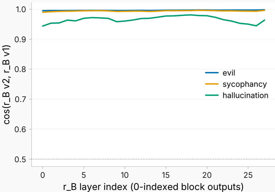
Direction stability under the faithful recipe
