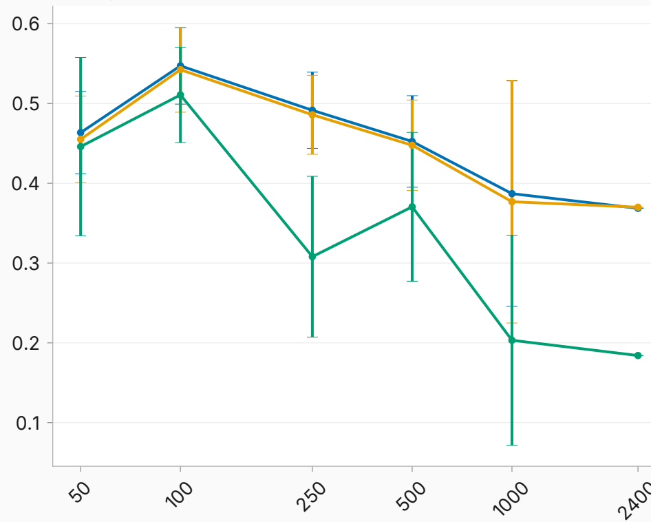
sycophancy — many-shot (L26)
