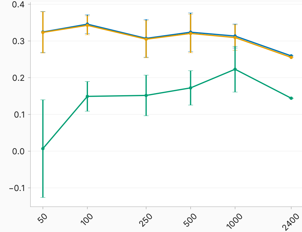
hallucination — many-shot (L27)
