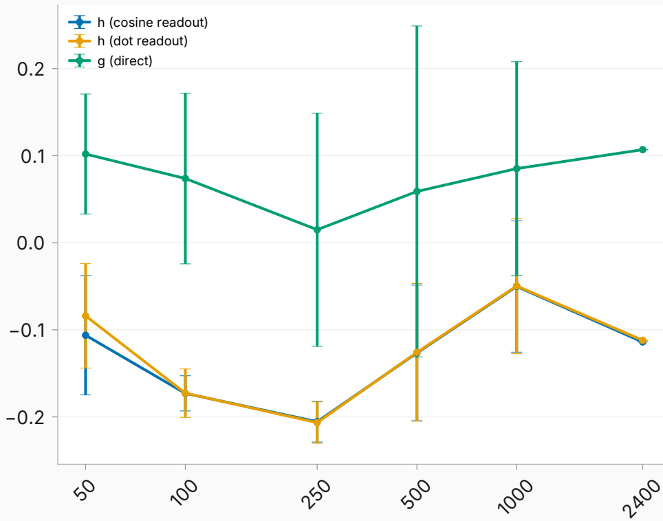
evil — many-shot (L26)
