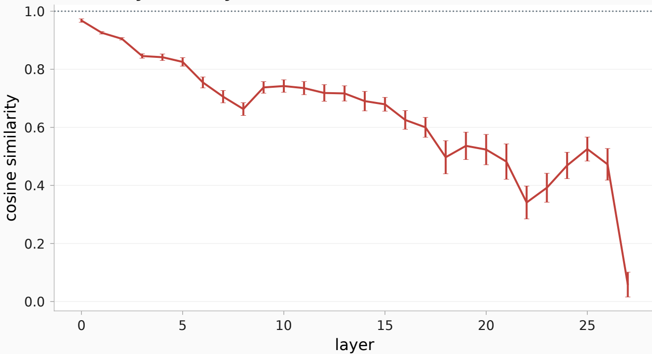
Boundary-triviality: turn-end newline vs context vector (mean \pm std over contexts)
