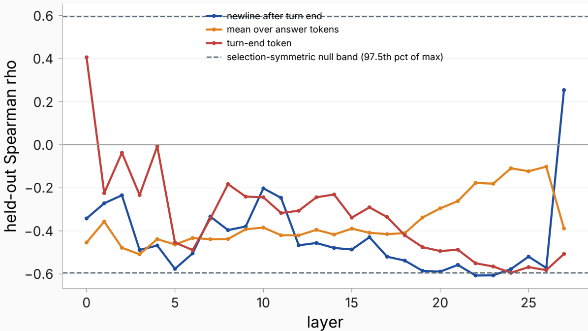
Refusal read-out along the fixed behavior direction, per layer (n = 50)
