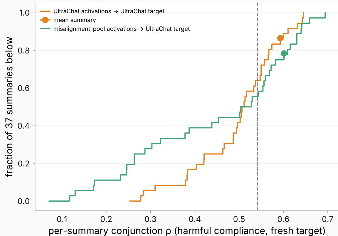
Harmful compliance: 13-16 of 37 summaries clear the band
