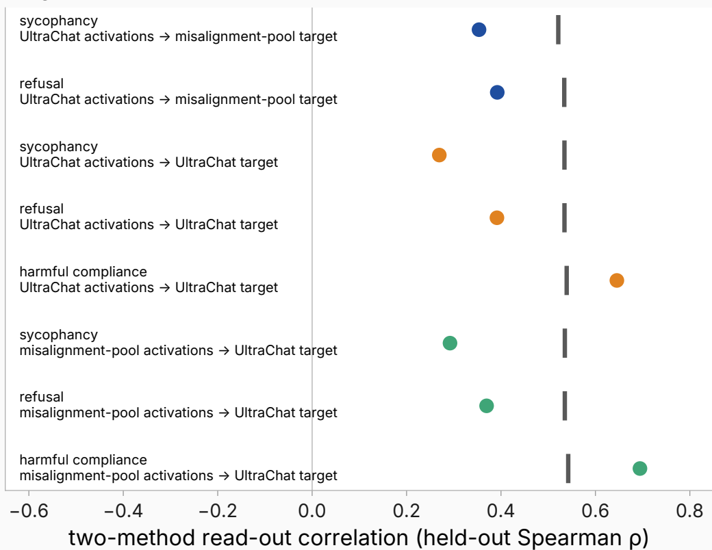
8 registered reads: observed (dot) vs null band (tick)
