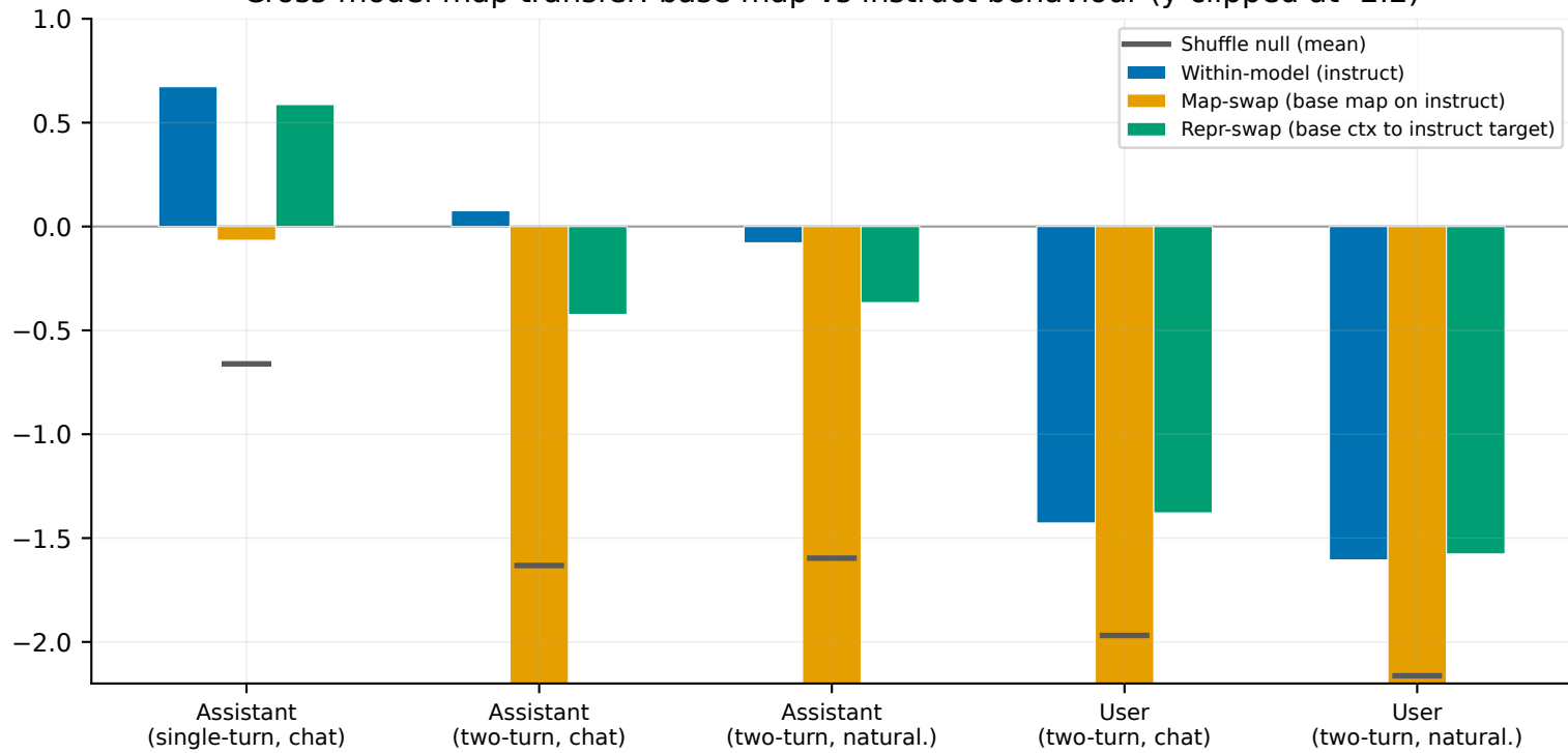
Cross-model map transfer: base map vs instruct behaviour (y clipped at -2.2)
