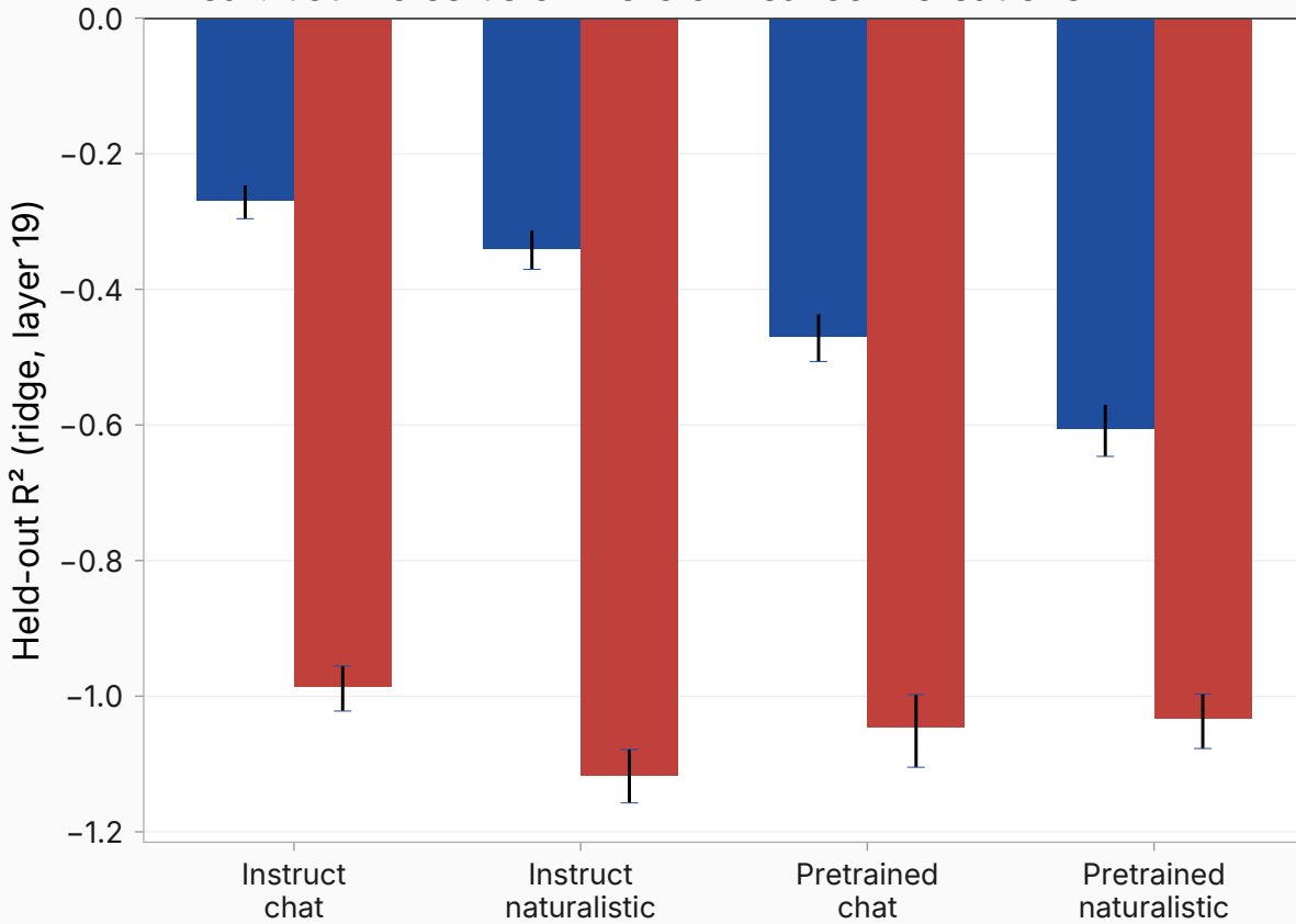
Linear: both roles below zero on real conversations
