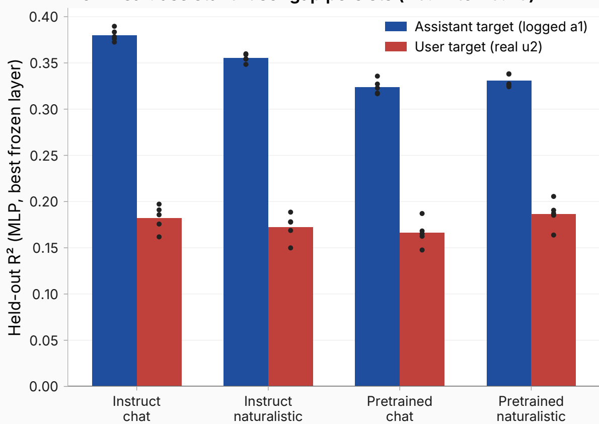
Nonlinear: assistant-user gap persists (+0.14 to +0.20)
