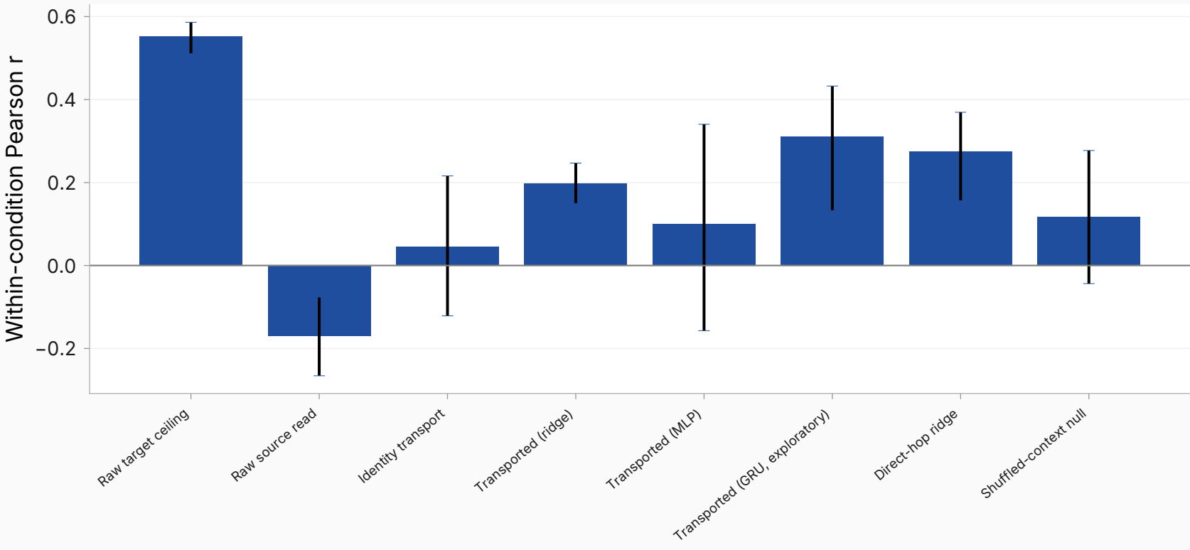
sycophancy — primary \ell^*=26 — many_shot (source layer 0)
