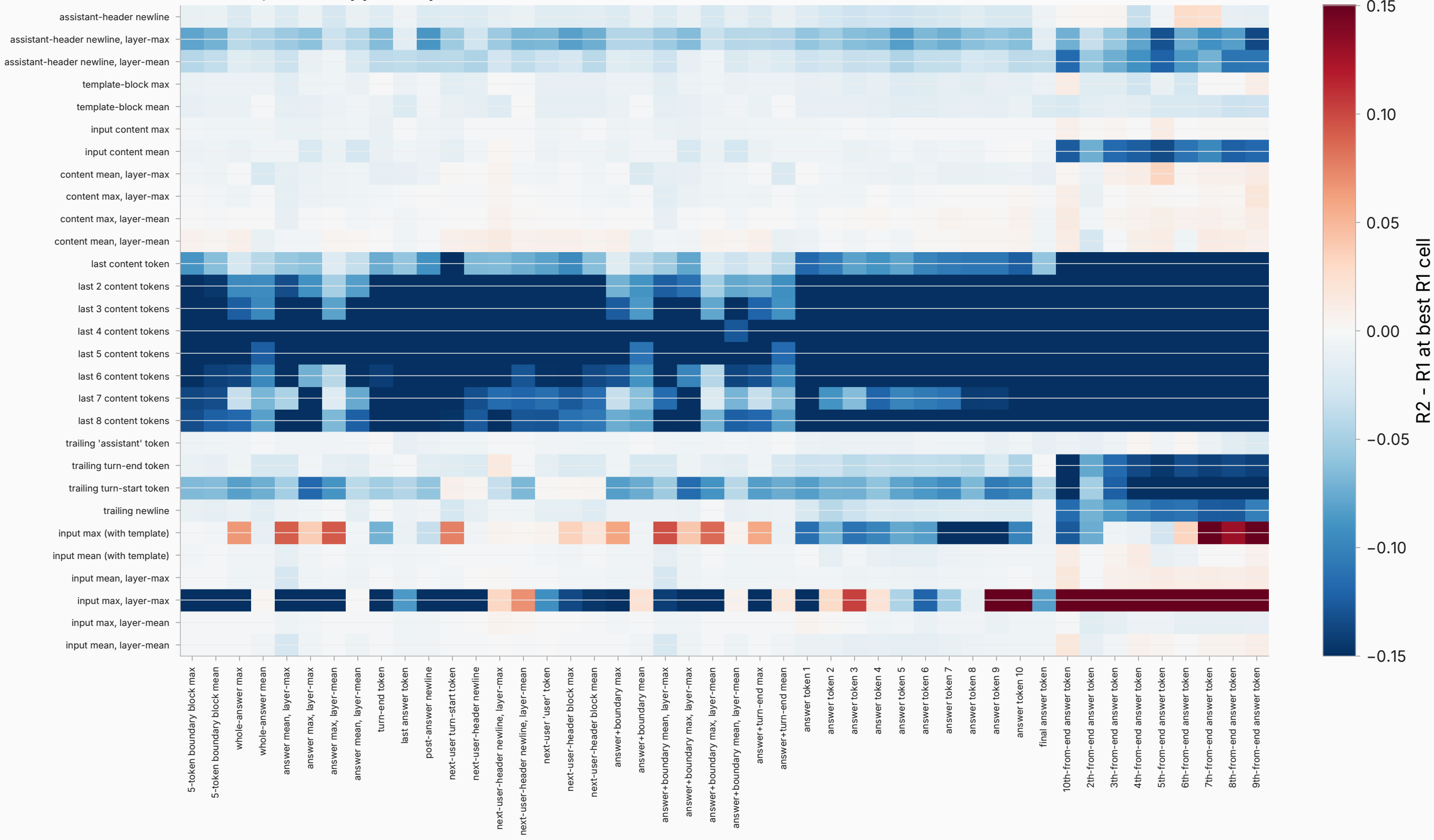
Probe-set generalization delta (input-OOD minus in-probe skill) at each family pair's best cell; color clipped to plus/minus 0.15
