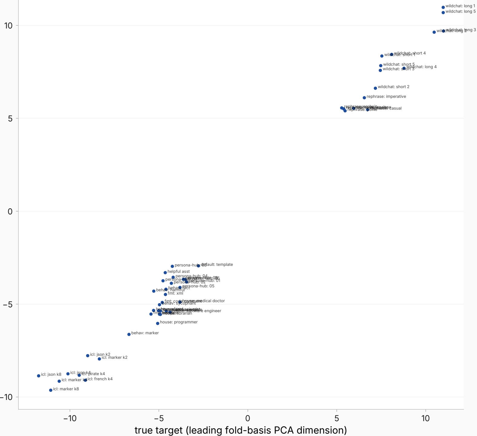
Winning map cell: context template-block max → answer user-header pool max, layer 12
