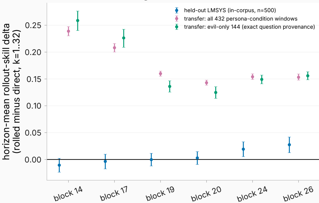
Recursion vs direct maps: in-corpus tie, clear rolled advantage on transfer
