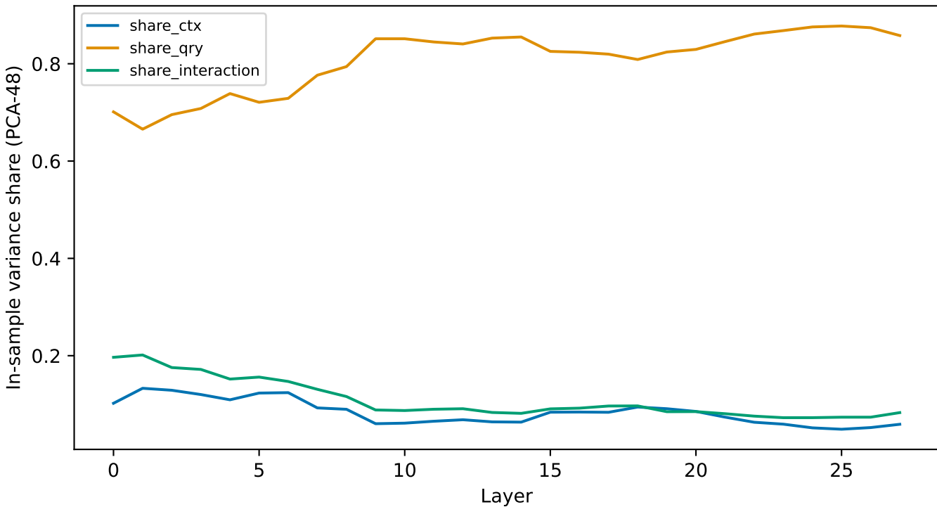
ANOVA oracle shares — betley (in-sample reference)
