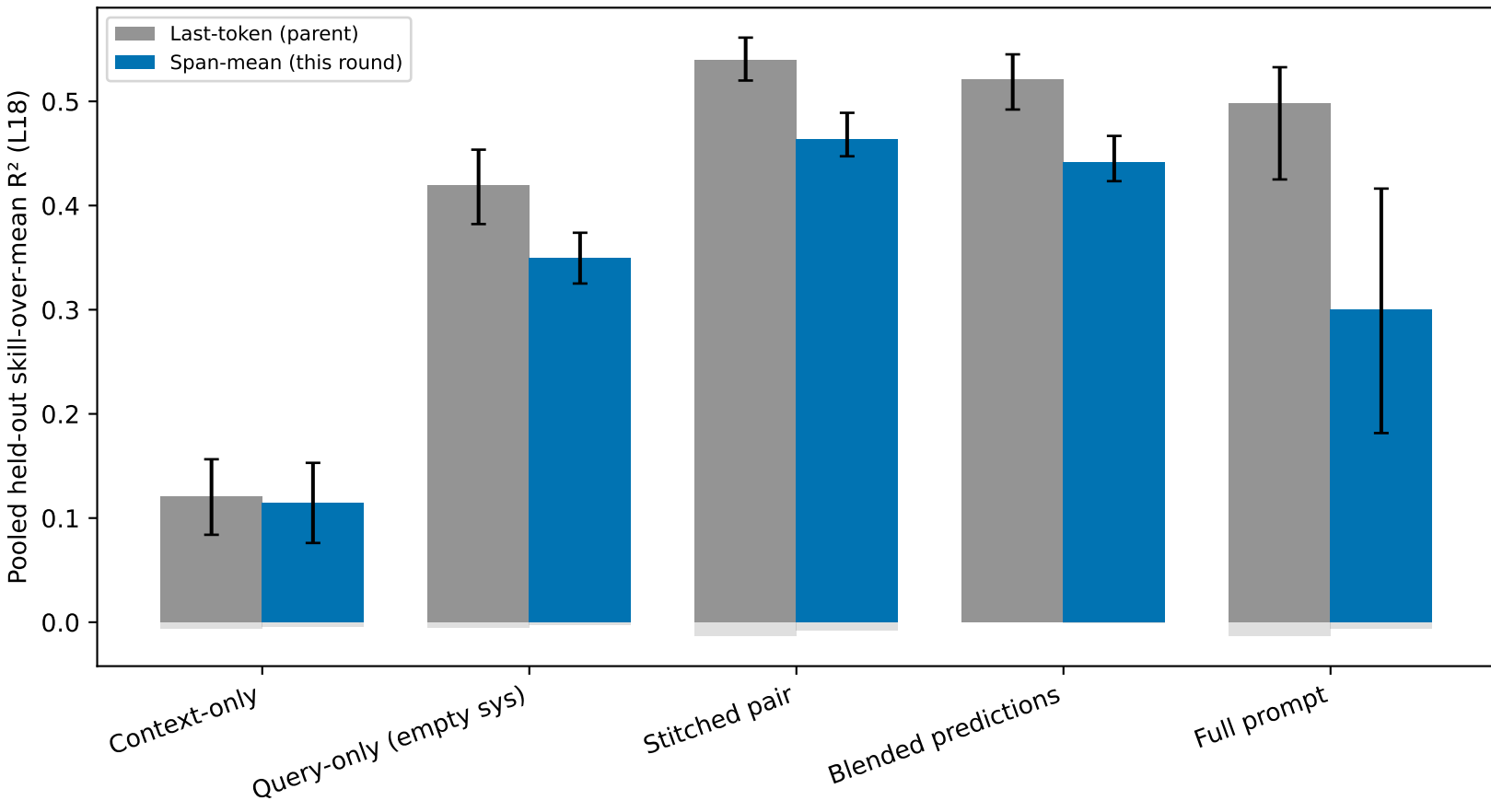
Last-token vs span-mean features — betley
