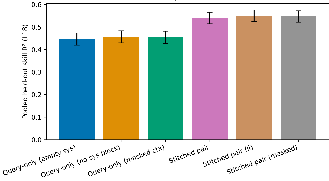
Null-context presentations — uc
