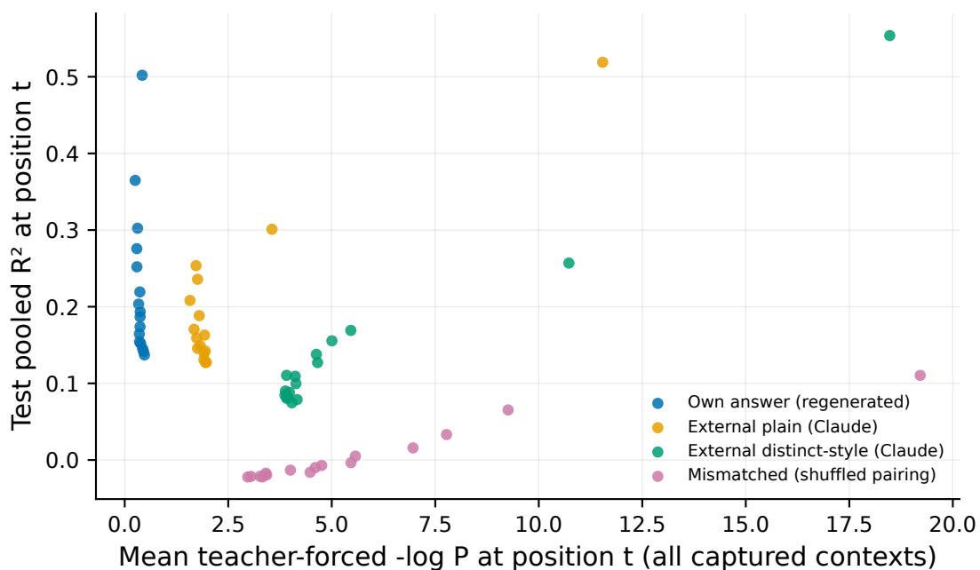
Predictability vs token-level surprise per position
