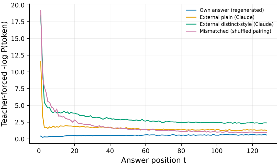
Token-level surprise per arm
