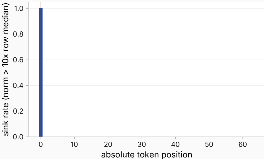
per-position sink rate (accent = map sink set, n=1)
