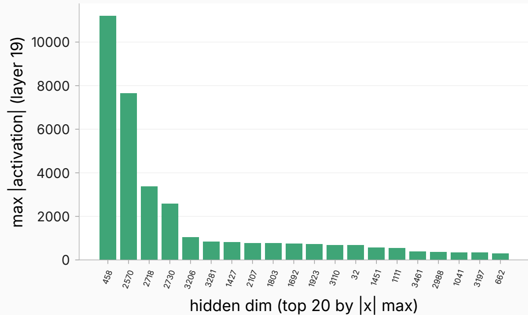
massive-activation dims — gamma=0.151
